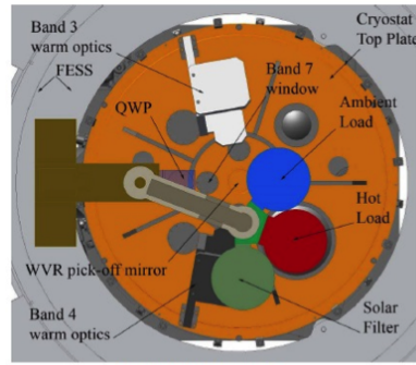
Figure 35: Calibration Device top view
