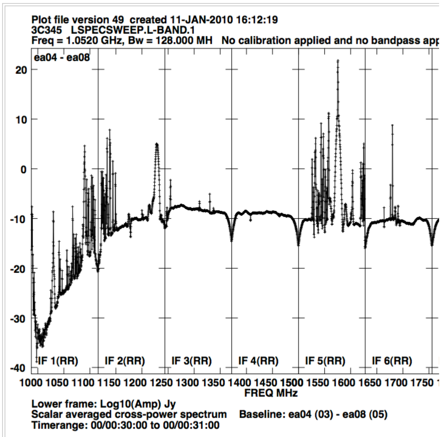
Figure 3: Spectrum of L-band RFI. This shows the major interfering signals seen across the full 1 G L-band receivers. Each of the eight “spectral windows” displays 128 MHz from a separate sub-band uncalibrated for the bandpass of either the digital filter or the receiver. The high linearity of the EV will permit astronomical observing within any frequencies not containing external interference. No units (dB).
