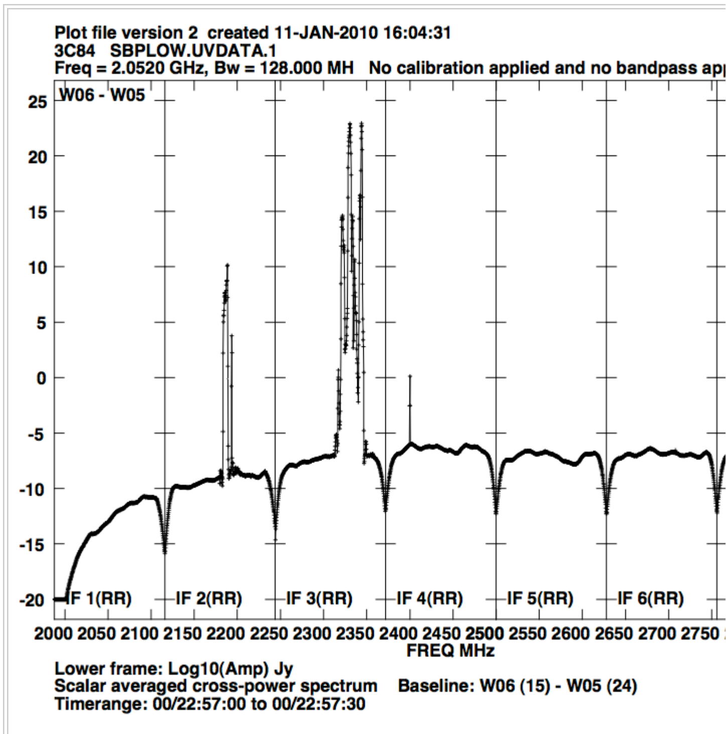
Figure 4: Spectrum of S-band RFI. This shows the raw spectrum of the lower half of S-Band – 2.0 to 2.75 GHz – as seen in the upper half. The major interference at 2.35 GHz is from satellite radio. The y-axis is in log
