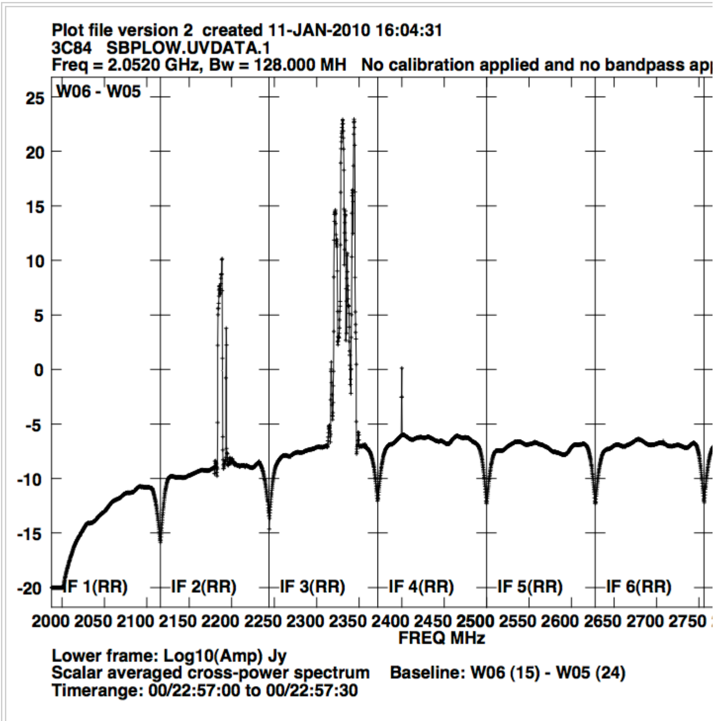
Figure 4: Spectrum of S-band RFI. This shows the raw spectrum of the lower half of S-Band – 2.0 to 4.0 GHz – seen in the upper half. The major interference at 2.35 GHz is from satellite radio. The y-axis is in log
