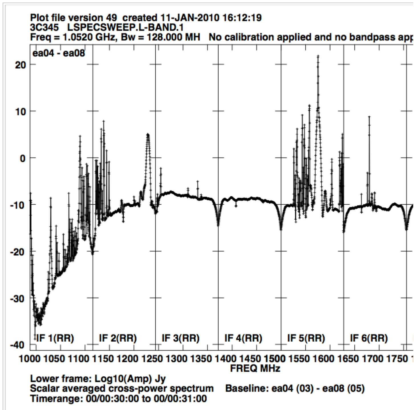
Figure 3: Spectrum of L-band RFI. This shows the major interfering signals seen across the full 1 GHz L-band receivers. Each of the eight “spectral windows” displays 128 MHz from a separate sub-band uncalibrated for the bandpass of either the digital filter or the receiver. The high linearity of the EVLA will permit astronomical observing within any frequencies not containing external interference. No units (dB).
