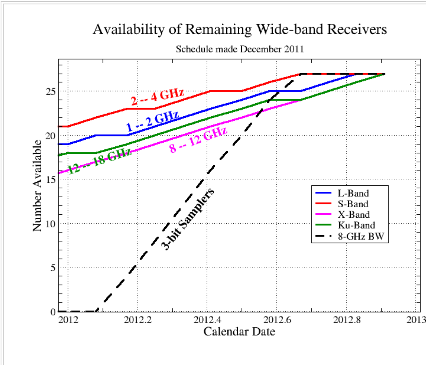
Figure 1: EVLA Receiver Deployment Plan. Above is a plot of the availability of final EVLA receivers the calendar year 2012 until the end of the EVLA Construction Project on December 31, 2012. Inter receivers with reduced frequency coverage or polarization purity are available at some bands in ad those plotted (see Table 4).
