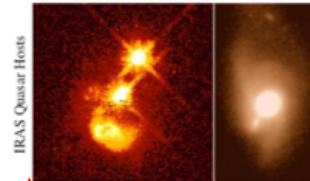
(e) "Blowout"
