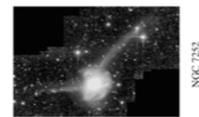
(g) Decay/K+A
