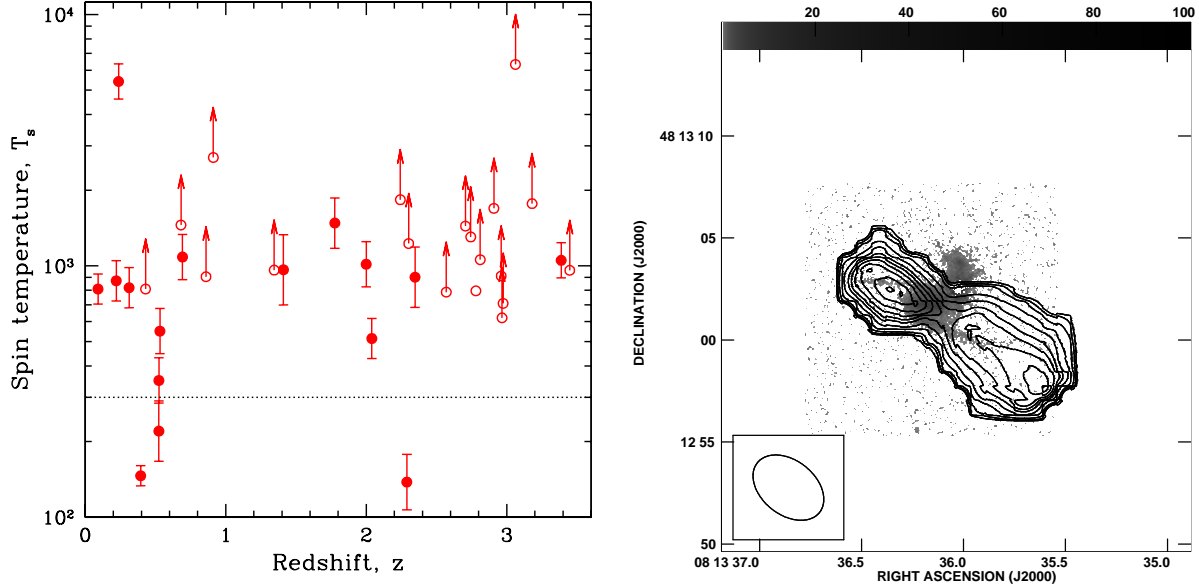
Figure 1: [A] Left panel: The spin temperature T_s plotted against DLA redshift for the 32 DLAs with T_s estimates (Kanekar et al. 2009a). The dashed horizontal line is at T_s = 300 K; 90% of Galactic sightlines show T_s < 300 K (Braun & Walterbos 1992). [B] Right panel: The contours show the integrated HI 21cm optical depth from the z \sim 0.437 DLA towards 3C196, overlaid on a Hubble Space Telescope (HST) image (in greyscale; Ridgway & Stockton 1997, AJ, 114, 511)
