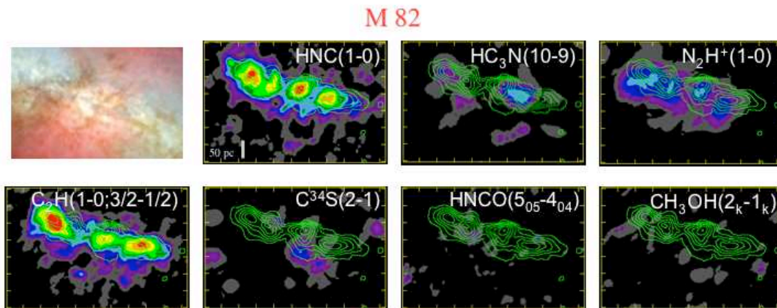
Figure 4: Same as in Figures 2-3 except for the much stronger starburst, M 82. Here the PDR species dominate, penetrating the entire ISM (Turner & Meier 2008).
