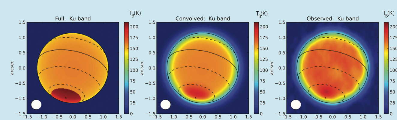
Figure 6. Chemical atmospheric models of Neptune compared to VLA observations. Adapted from Fig. 19 of [7].
