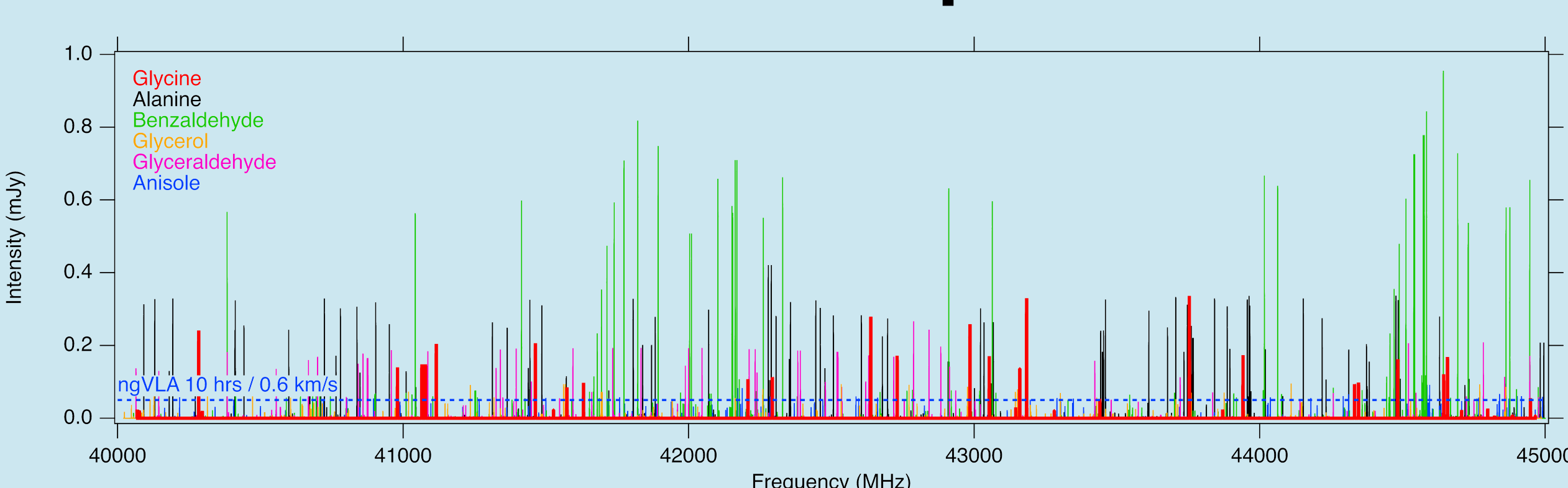
Figure 7. Simulation of the kinds of complex molecules that will be detectable with the ngVLA, but which are not observable with modern facilities in a practical integration time.
