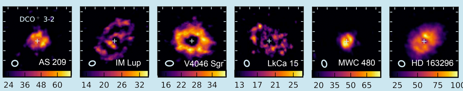
Figure 1. ALMA observation of DCO + emission across six different protoplanetary disk sources. Adapted from Fig. 1 of [3].
