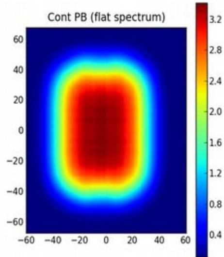
Mosaic PB Sensitivity
