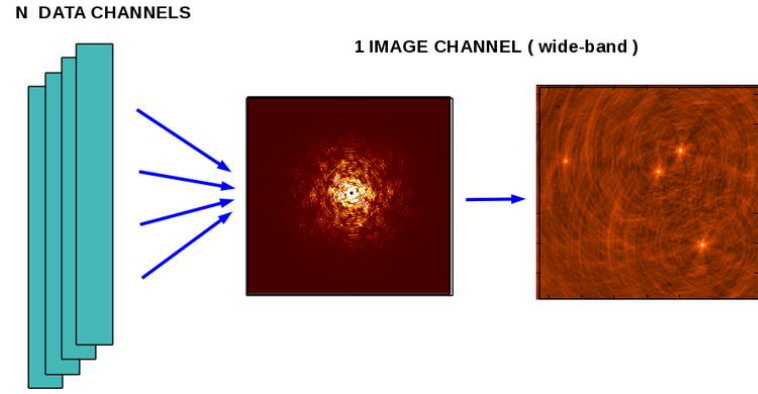
Continuum Imaging specmode='mfs'
