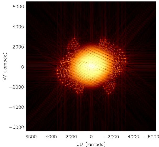
Visibilities (complex)
