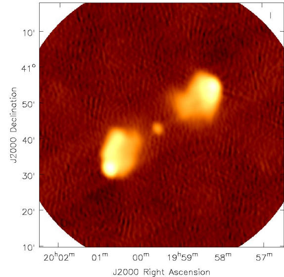
Sky Brightness (Real)
